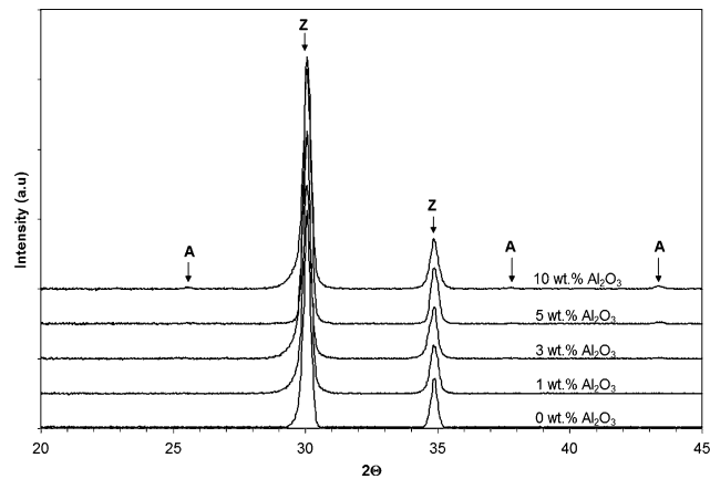
Fig. 2 X-ray diffraction patterns for 8Y-CSZ + 5 wt. % \text{SiO}_2 with varying amounts of \text{Al}_2\text{O}_3 prior to deformation. Specimens were sintered at 1200 °C for 3 h. Z = 8Y-CSZ. A = \text{Al}_2\text{O}_3
