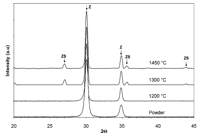
Fig. 3 X-ray diffraction patterns for 8Y-CSZ + 5 wt. % \text{SiO}_2 + 1 wt. % \text{Al}_2\text{O}_3 . The specimen at 1200 °C was sintered for 3 h; all others were sintered for 1 h. Z = 8Y-CSZ. ZS = \text{ZrSiO}_4
