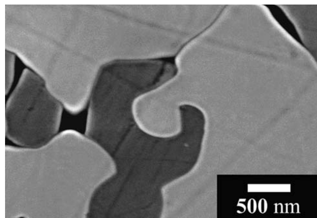
Fig. 8 Locking microstructure of \text{ZrSiO}_4 (dark gray) and 8Y-CSZ (light gray) formed after high temperature heat treatment of 1450 °C, 1 h
