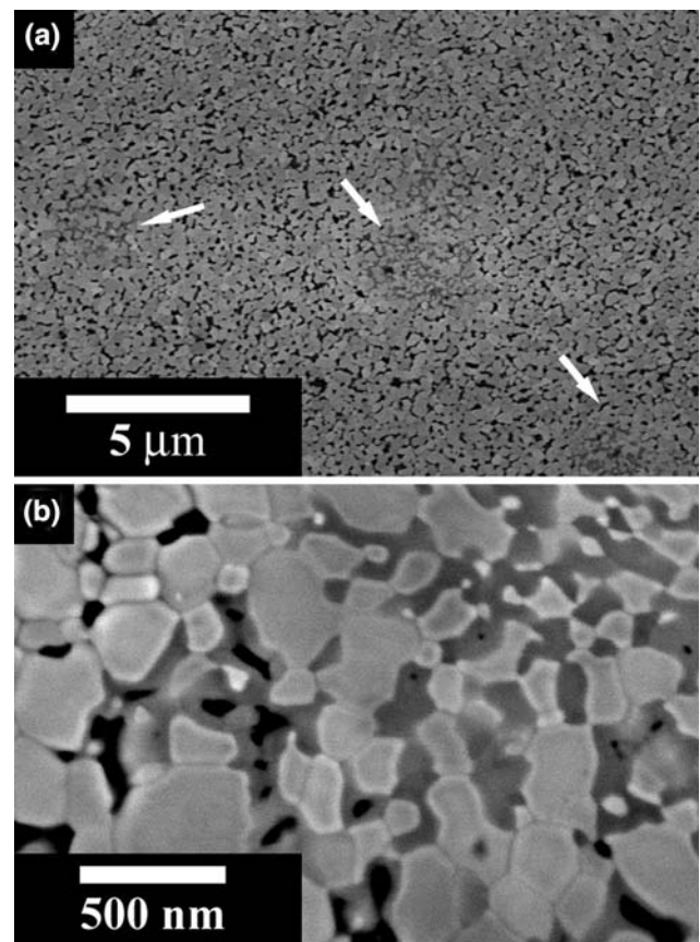
Fig. 5 Formation of \text{ZrSiO}_4 after deformation of 8Y-CSZ/ \text{SiO}_2 with 1 wt.% \text{Al}_2\text{O}_3 . (a) Inhomogeneous crystallization of \text{ZrSiO}_4 . (b) Reaction between 8Y-CSZ and \text{SiO}_2 . Light gray is 8Y-CSZ, gray is \text{ZrSiO}_4 , and black is \text{SiO}_2
